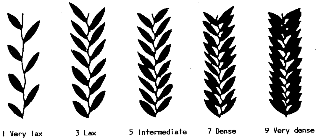
Fig. 1. Spike density
